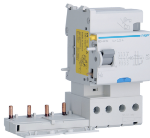
BD441N
